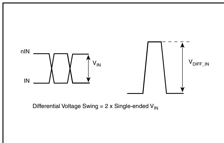
Single-Ended & Differential Input Voltage Swing
