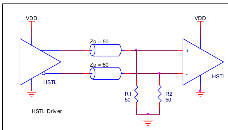
Figure 4. Output Termination
