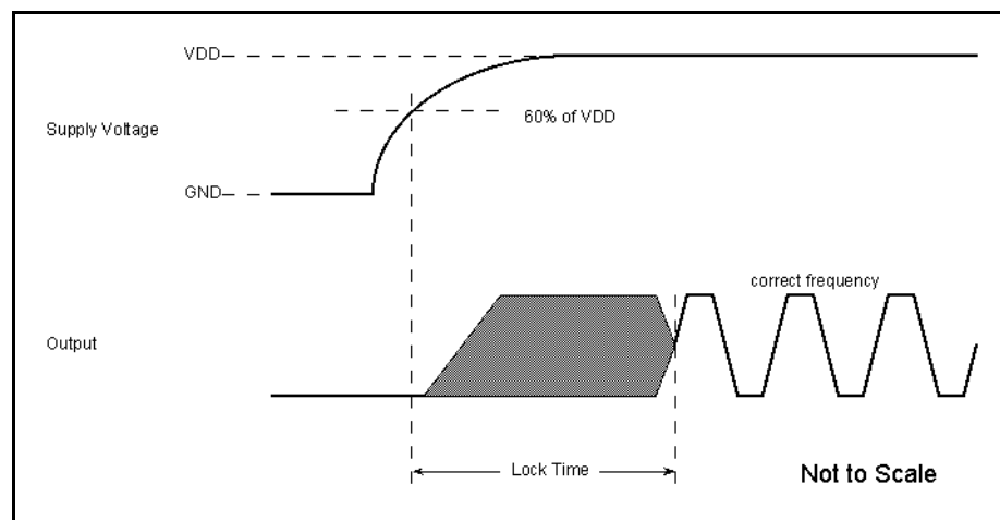
PLL Lock Time
