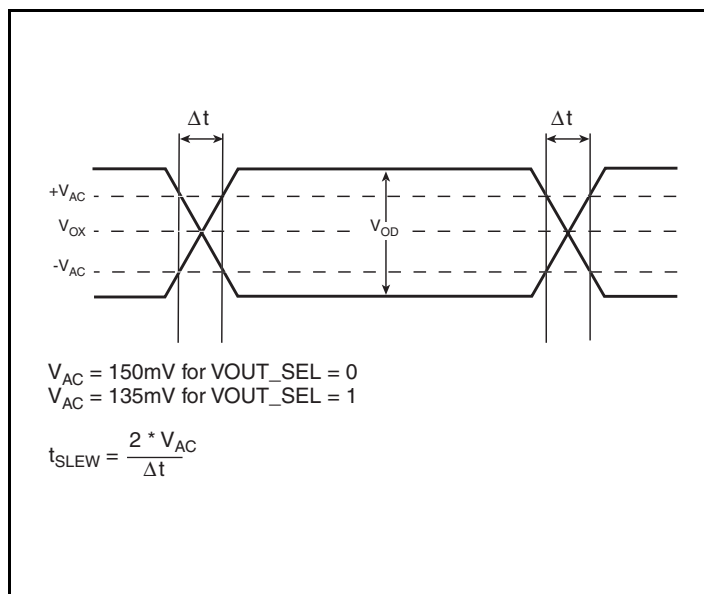
Slew Rate
