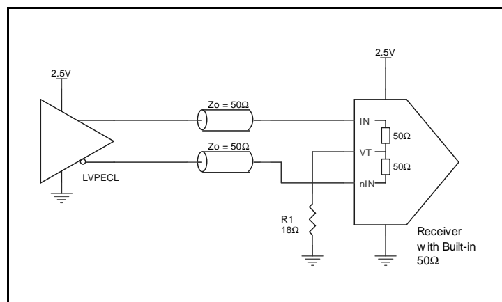
Figure 4C. IN/nIN Input with Built-In 50Ω driven by an LVPECL Driver
